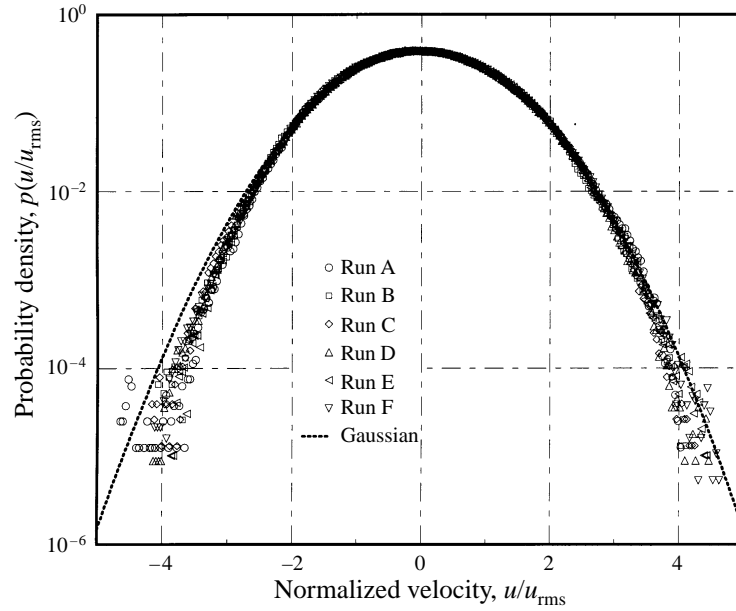
FIGURE 4. PDF of streamwise velocity normalized by u_{\text{rms}} for the six runs. A reference Gaussian is shown.
